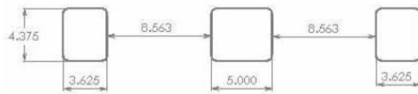
Cutouts for 760 Series Devices
